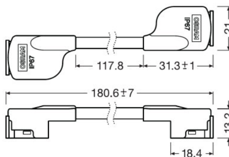
JUMPER-FLEX-IP67-2P
