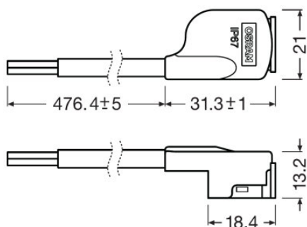
CONN-FLEX-IP67-2P
