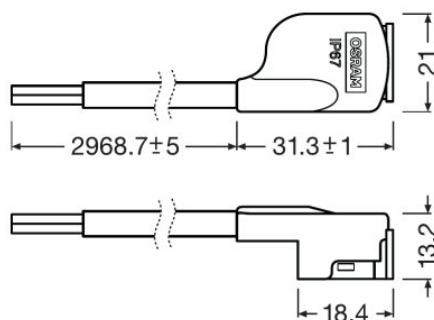
CONN-FLEX-IP67-2P-300
