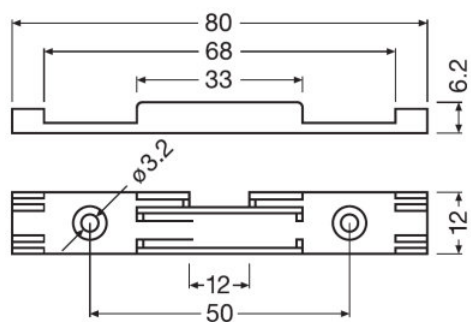
LR700SD-G1- PLATE FOR MAGNET
